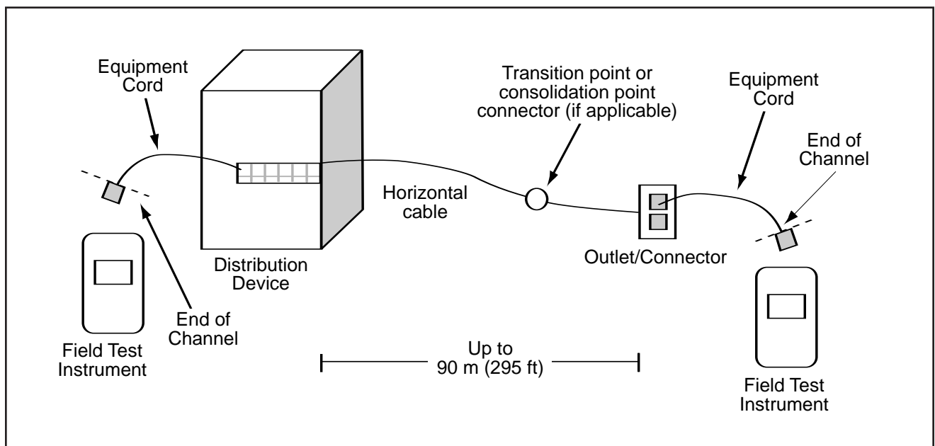
Figure 24—Channel test configuration
