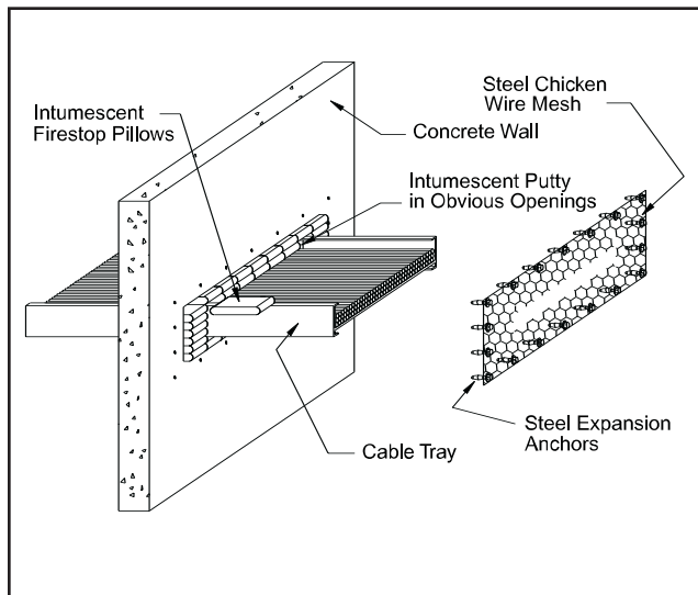
Figure 18—Fire seal cable tray penetration
