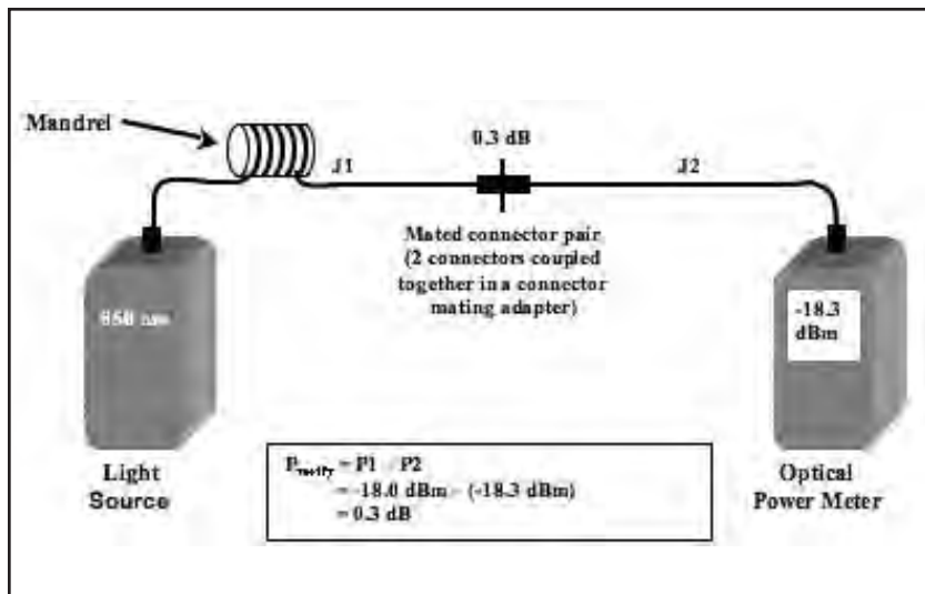
Figure 26—Example of a measurement ( P_2 ) when verifying OLTS test jumpers (multimode)
