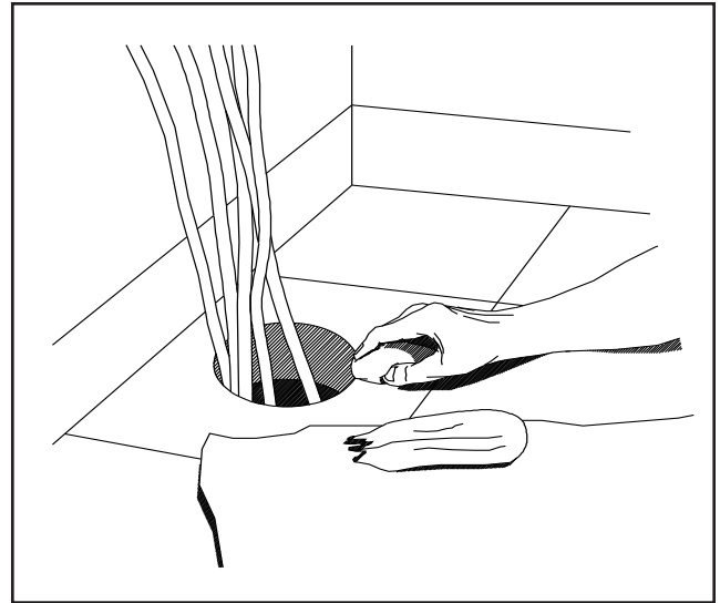
Figure 10—Building bottom of penetration seal
