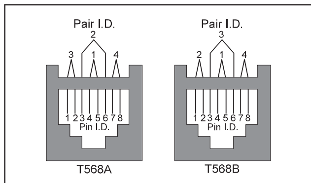
Figure 19—Wiring schemes
