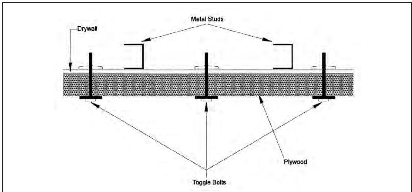
Figure 8—Plywood installation over drywall using toggle bolts
