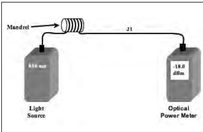
Figure 27—Example of OLTS reference measurement ( P_1 ) with one test jumper (multimode)
