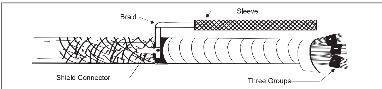
Figure 20—Shield bond connector and braid
