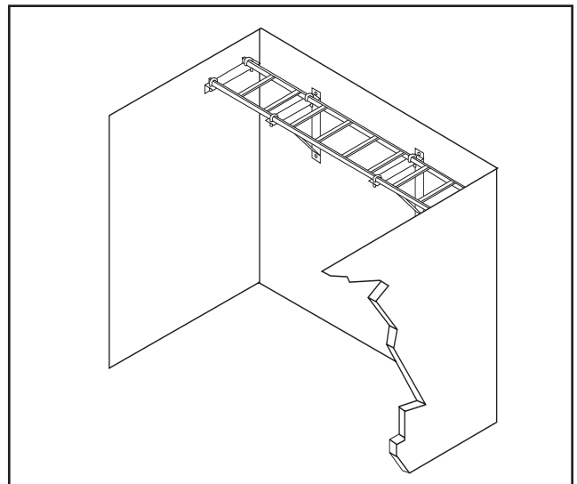
Figure 5—Elevation view of cable tray installed on the rear wall of a telecommunications room
