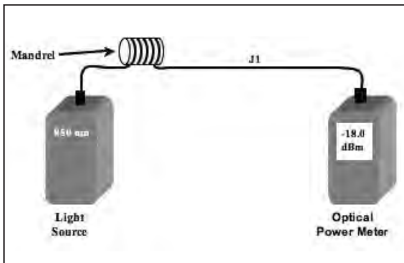
Figure 25—Example of OLTS reference measurement ( P_1 ) with one test jumper (multimode)
