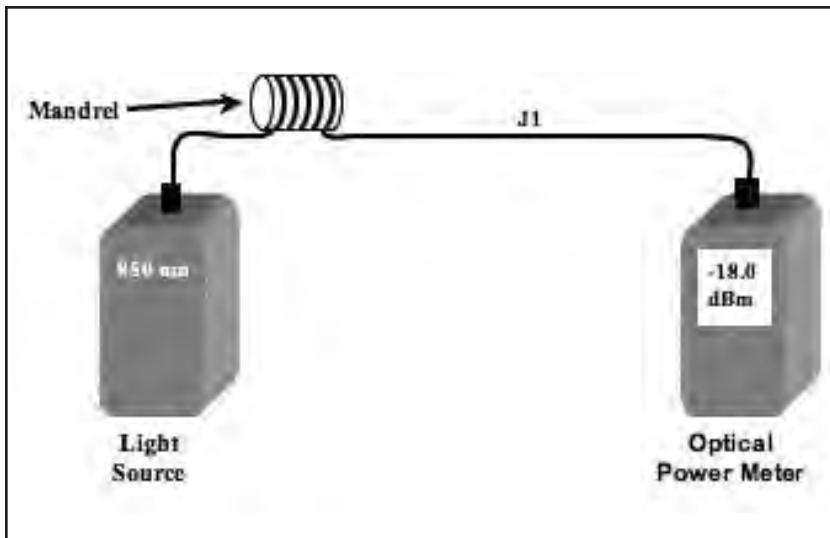
Figure 28—Example of a multimode link attenuation measurement ( P_2 )
