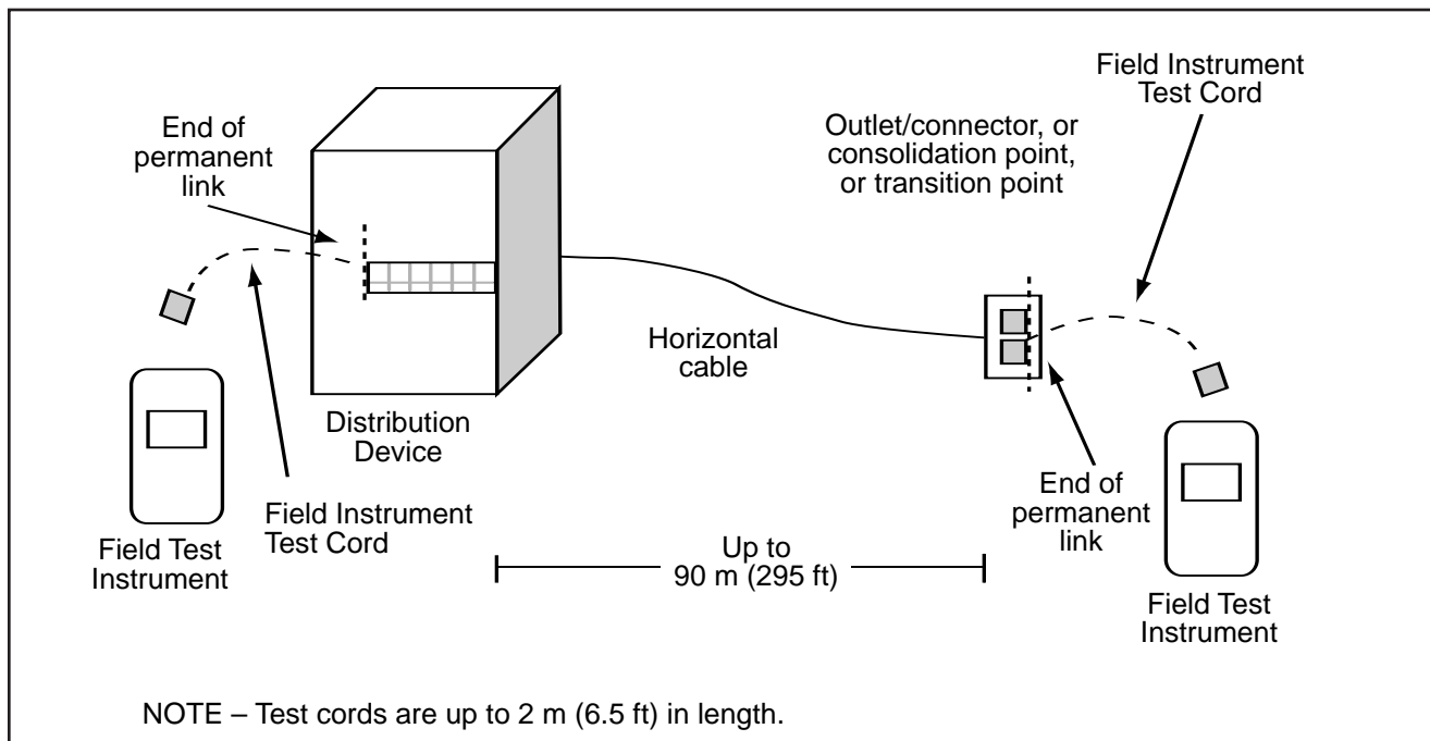
Figure 23—Permanent link test configuration
