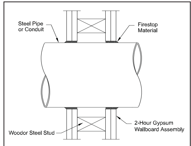
Figure 17—Fire seal of drywall
