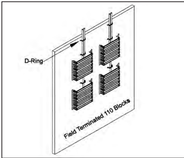
Figure 6—Typical backboard layout using distribution-rings
